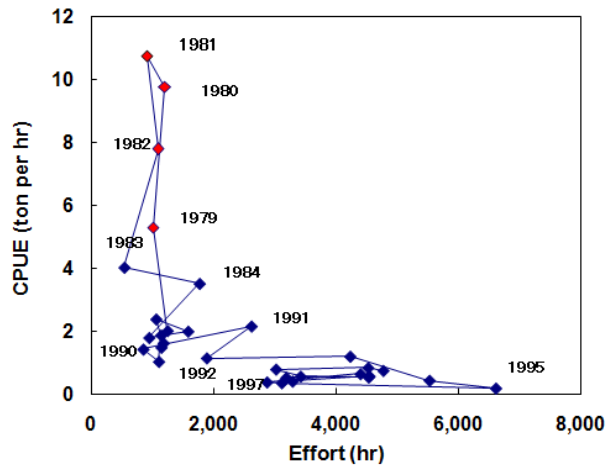
Fig. 9. Excel Solver run output with adjusted CPUE. Relationship between fishing effort and adjusted CPUE
